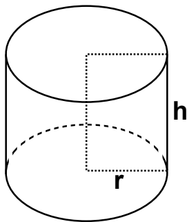
Cylinder
