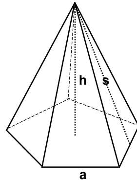
Regular Pyramid on Polygonal Base (n=5)
