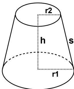
Frustum of a Cone
