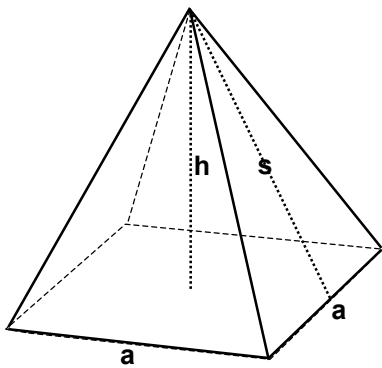
Regular Pyramid on Square Base
