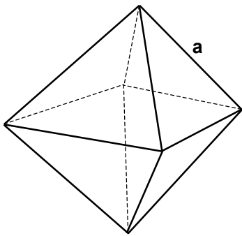
Regular Octahedron
