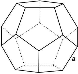
Regular Dodecahedron
