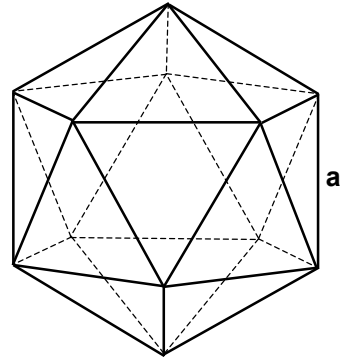
Regular Icosahedron
