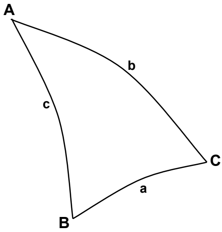
Spherical Triangle
