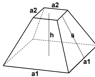
Frustum of a Pyramid (square base)
